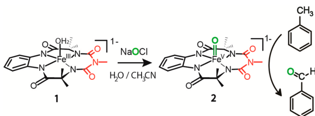
Scheme 1. Formation of \text{Fe}^{\text{V}}(\text{O}) Species in an \text{H}_2\text{O}/\text{CH}_3\text{CN} Mixture and Its Reaction toward Toluene
