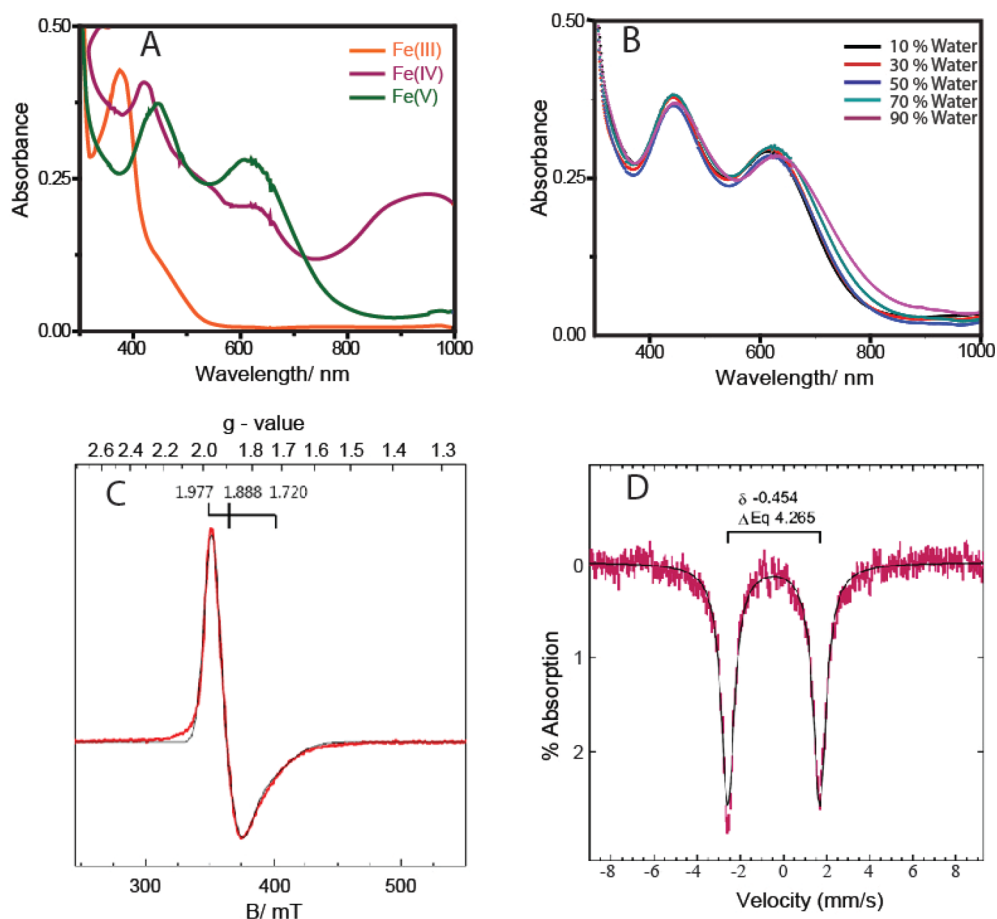
Figure 1. (A) UV-vis spectral changes of 1 ( 10^{-4} M) (orange) upon the addition of 0.5 equiv of NaOCl ( 5 \times 10^{-5} M) in CH 3 CN, forming the \mu -Oxo-Fe IV dimer species (violet). Addition of another 0.5 equiv of NaOCl ( 5 \times 10^{-5} M) to the preformed \mu -Oxo-Fe IV dimer species produces the spectrum of Fe V (O) ( 2 , green). (B) UV-vis spectra of Fe V (O) in different H 2 O/CH 3 CN mixtures. (C) EPR spectra of Fe V (O) ( 2 ) in acetonitrile (2 mM) at 21 K. Black = experimental, red = simulated. (D) Mössbauer spectra of 57 Fe-enriched [Fe V (O)] ( 2 ) in acetonitrile (2 mM) at 4.2 K. The solid lines are spectral simulations.
